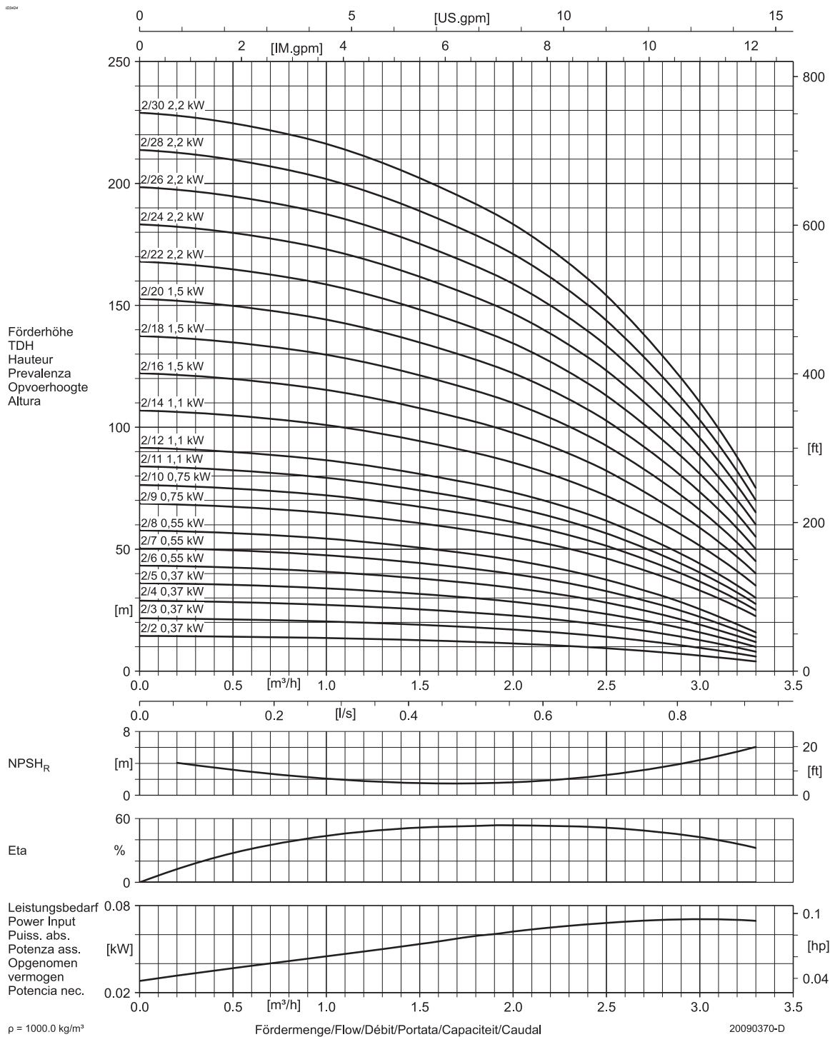
Figure 5: Performance curve DPVCI 2 B - 50Hz - 2 pole
